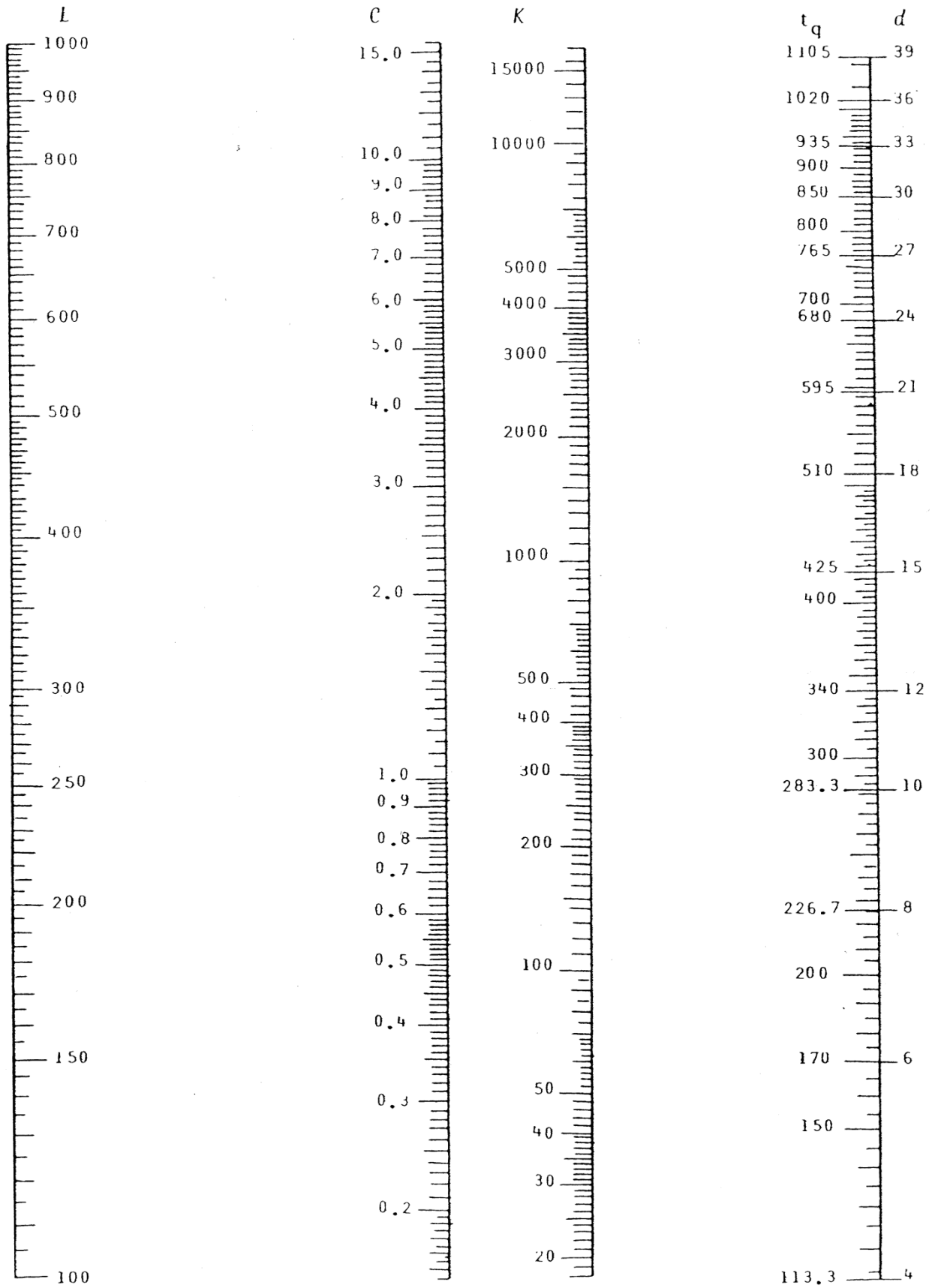
Nomograph for the solution of K = .011d^2L , C = .0003882dL , t_q = K \div C
